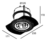
29810 0230 MOUNTING KIT TOP AIR 103
